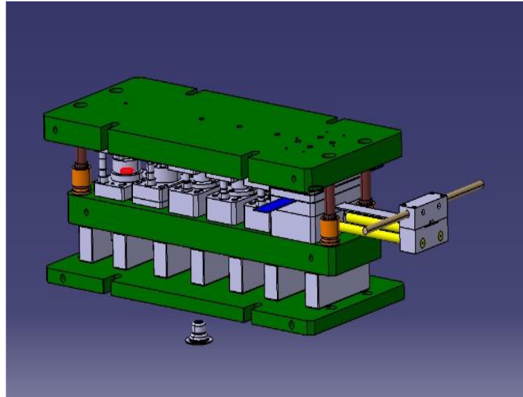
MOLD DESIGN
