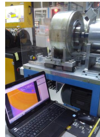
Thermal Camera
