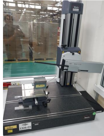
Contour Measuring
